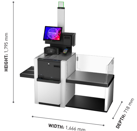
4 bagging variant Height: 1,795 mm Width: 1,666 mm Depth: 718 mm
