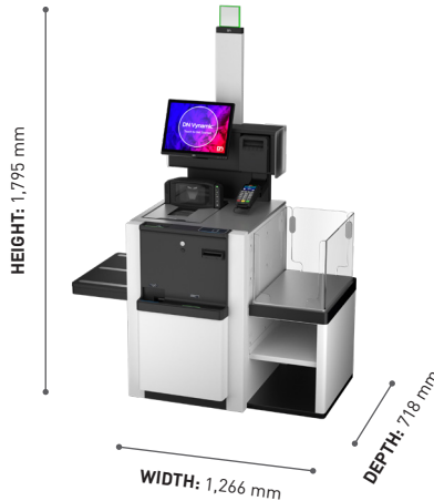
2 bagging variant Height: 1,795 mm Width: 1,266 mm Depth: 718 mm
